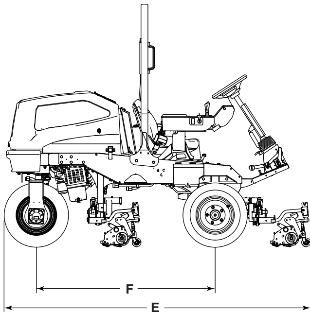
3WD Option Cutting Units Lowered Right Side View
