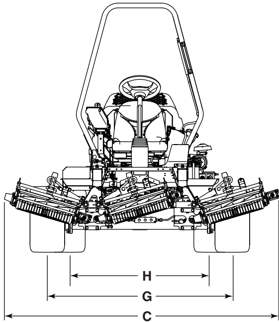
4WD Option Cutting Units Lifted Front View
