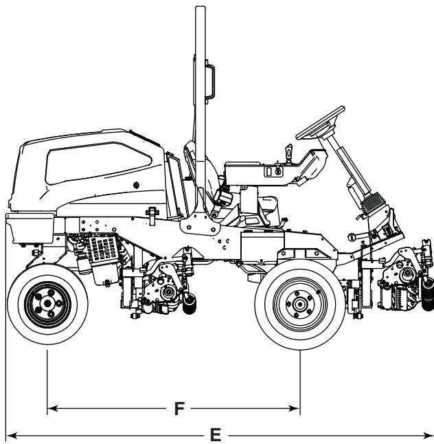
4WD Option Cutting Units Lifted Right Side View
