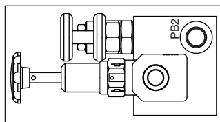
Brake Valve Viewed From Left
