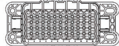
MODULE A & B: CAVITY NUMBERS (CABLE ENTRY VIEW)
