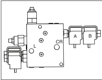
Lift Valve Viewed From Front
