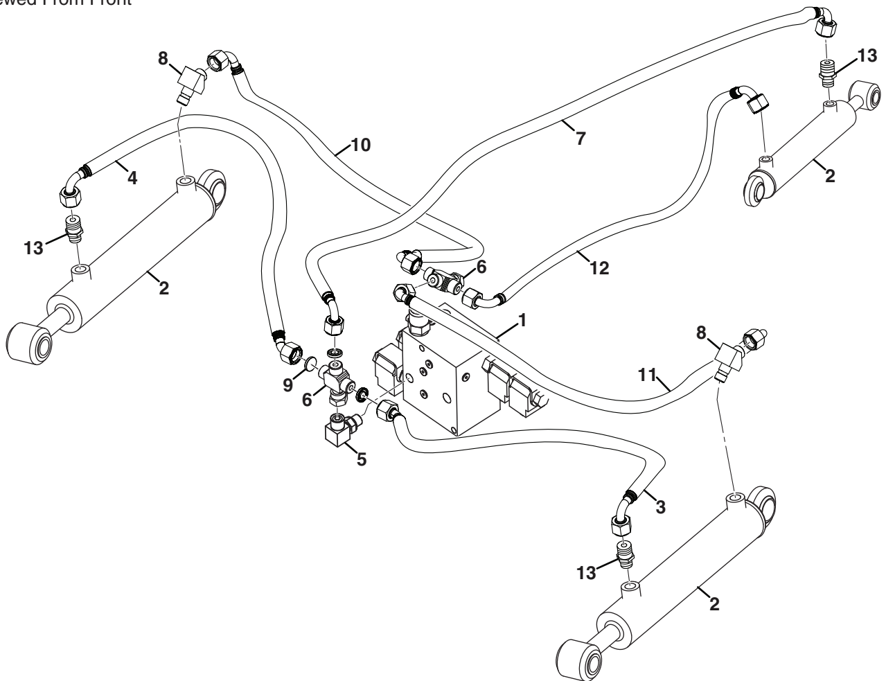
Lift Valve Viewed From Front
