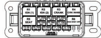
MODULE B: FUSE & RELAY LOADING VIEW (FUSES & RELAYS SUPPLIED WITH HARNESS)
