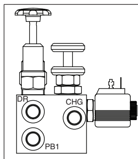
Brake Valve Viewed From Bottom
