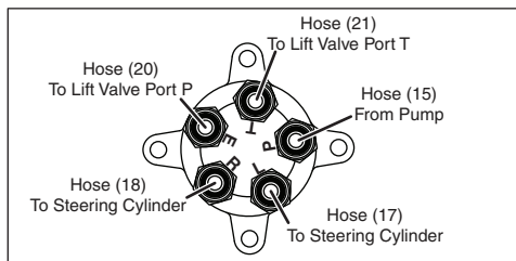
Steering Valve viewed from end
